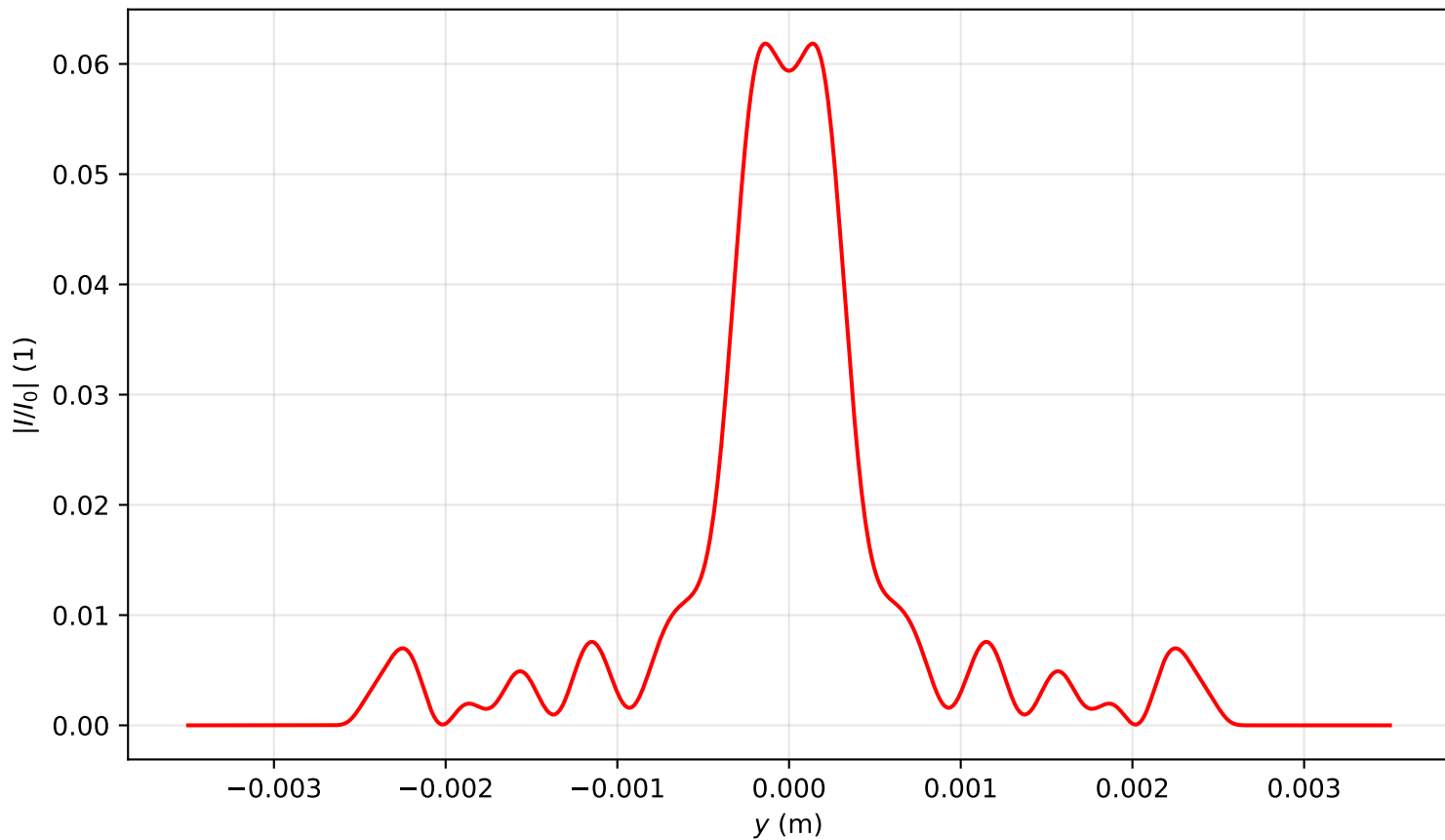
Intensity profile I(x = 0, y, z = 3.821)/I_0 , P_{in}=9.0P_{cr} , artificial time
